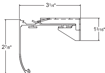
Color Coordinated Head Rail
