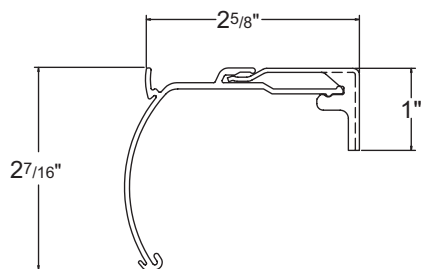
UltraSleek Head Rail
