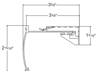
Deluxe Head Rail
